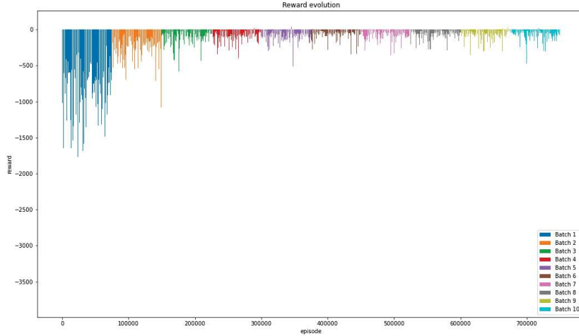
Figure 2: Reward evolution across batches (no transaction costs).
